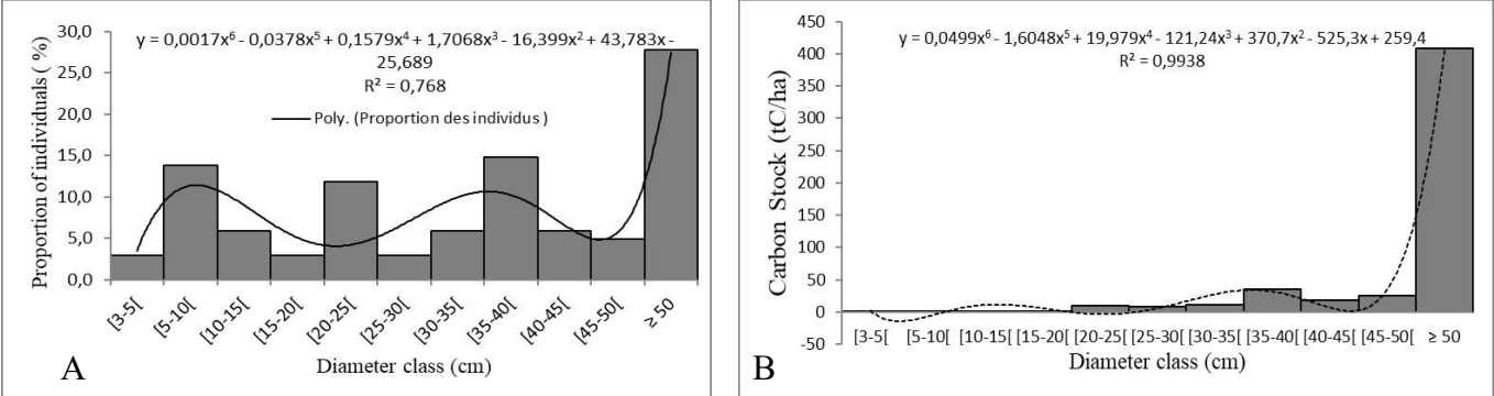
Figure 4. Distribution of individuals (A) and their carbon stock (B) by diameter class (Source: D. Gomis, 2019)
