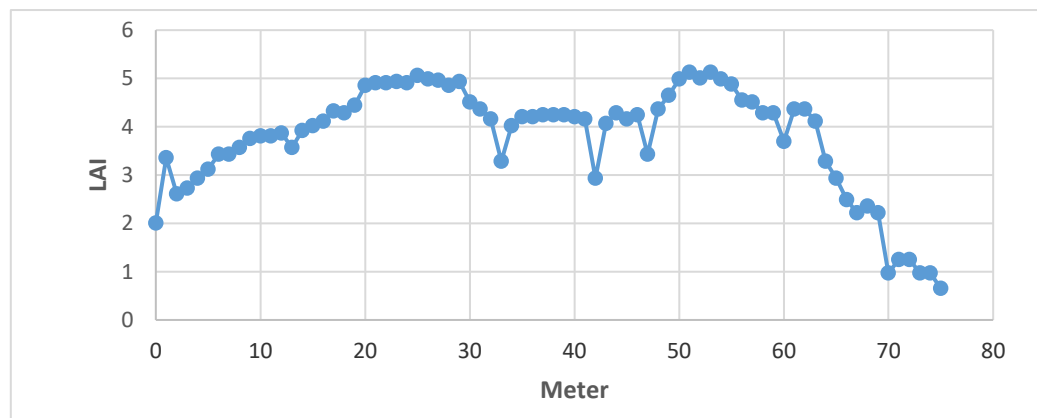
Figure 3: LAI variation per meter at Mangrove 1 site
